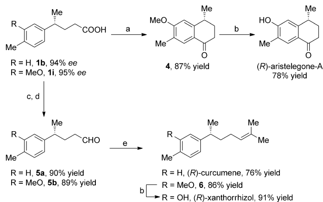
Scheme 4. Synthetic applications of hydrogenation products. Reaction conditions: a) trifluoroacetic acid, trifluoroacetic anhydride, 0 °C; b) \text{Et}_2\text{NCH}_2\text{CH}_2\text{SNa} , DMF, reflux; c) \text{CH}_3\text{I} , \text{K}_2\text{CO}_3 , DMF, RT; d) diisobutylaluminum hydride, \text{CH}_2\text{Cl}_2 , -78^\circ\text{C} ; e) (\text{CH}_3)_2\text{CH=PPh}_3 , THF, -15^\circ\text{C} .
